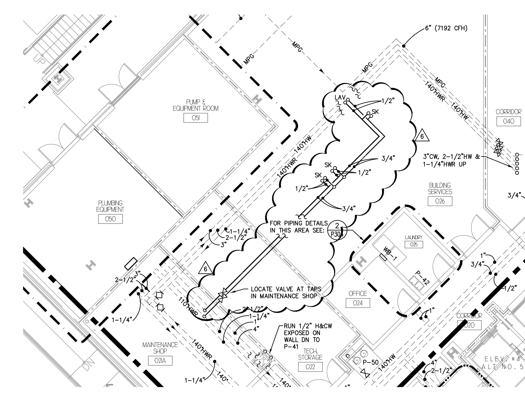
2 RETAIL #4 - PRESSURE PIPING P203 SCALE: 1/8" = 1'-0"
